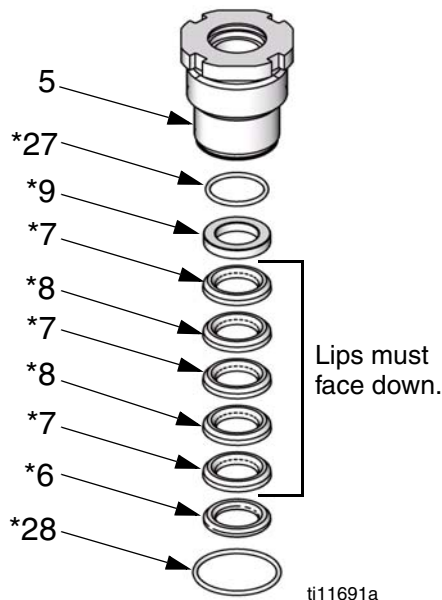
FIG. 3. Replace Throat Packings
